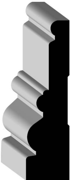
Casing 83488-97180 3/4" X 2-3/4"
