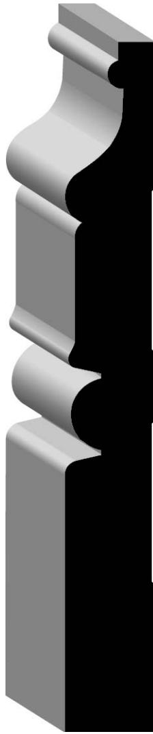
Baseboard 82168-97192 1 1/16 x 5-1/4
